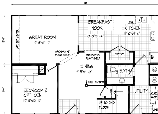
FIRST FLOOR PLAN MOD 2140-T APP. 1074 SF
