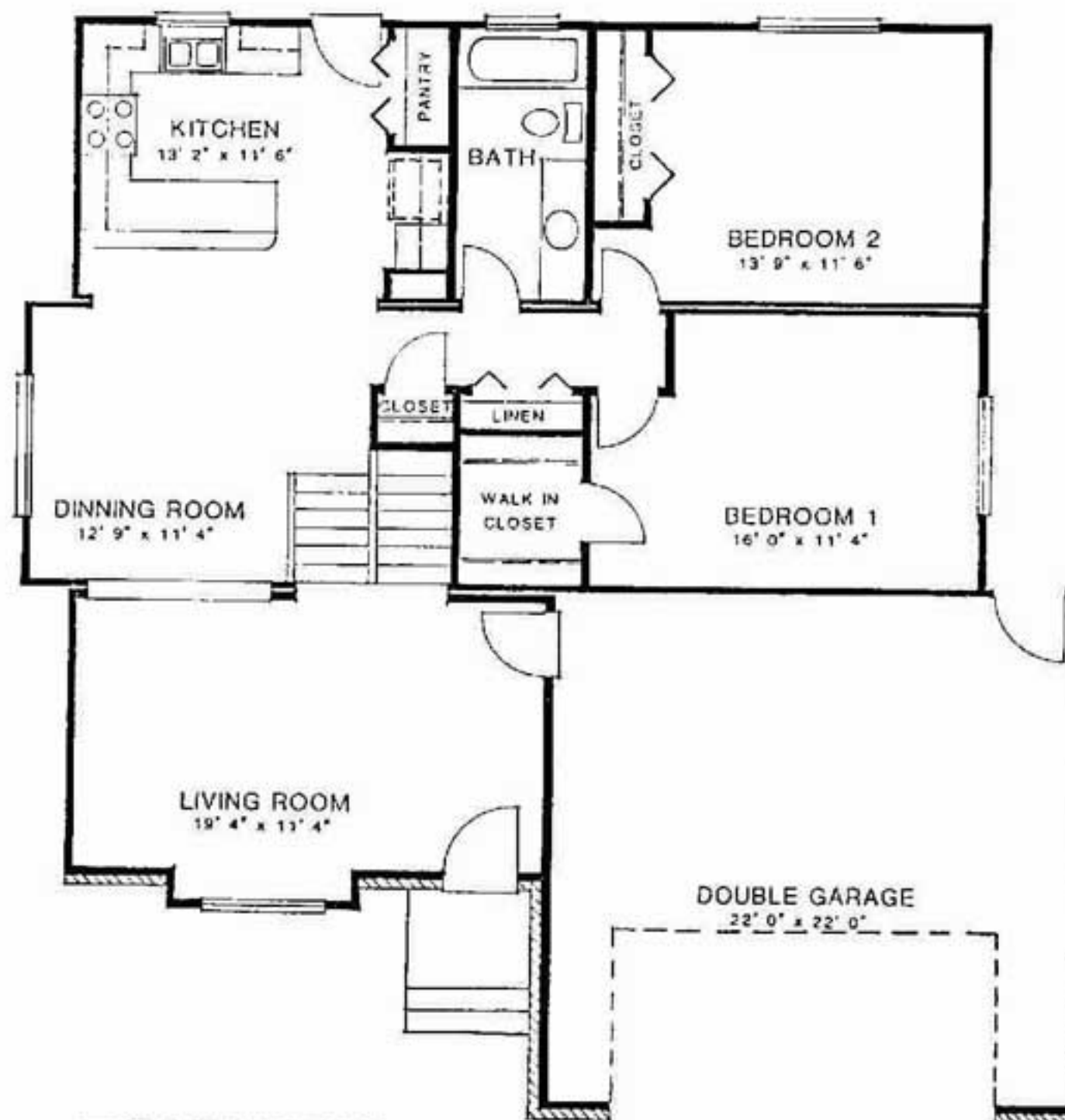
BOUNTIFUL TRI-LEVEL 36'-0" X 36'-2" — 1128 SQ. FT. 2 BEDROOMS — 1 BATH
